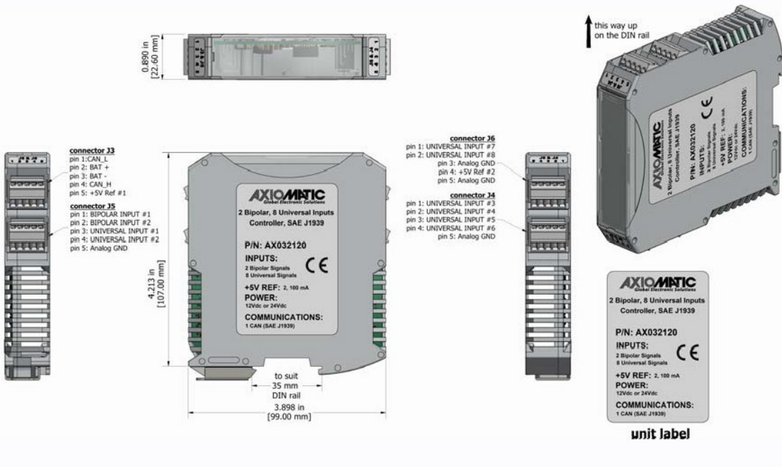
Figure 3.0 – Dimensions of AX032120
