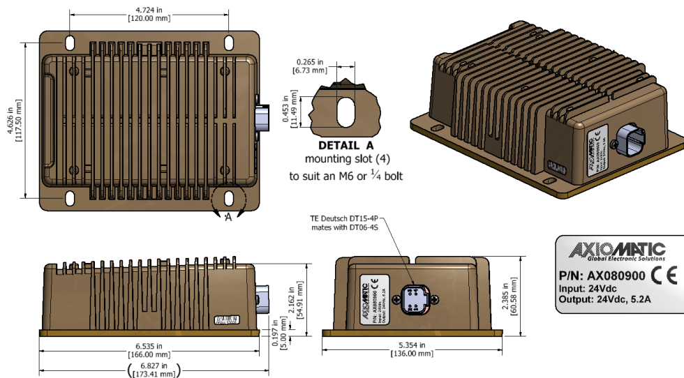
Figure 3.0 – Dimensional Drawing of AX080900 (AX080911 dimensions are the same.)
