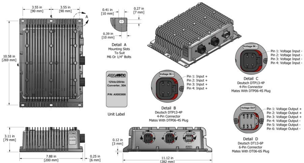
Figure 4. 0. – Dimensional Drawing of AX083800 Converter
