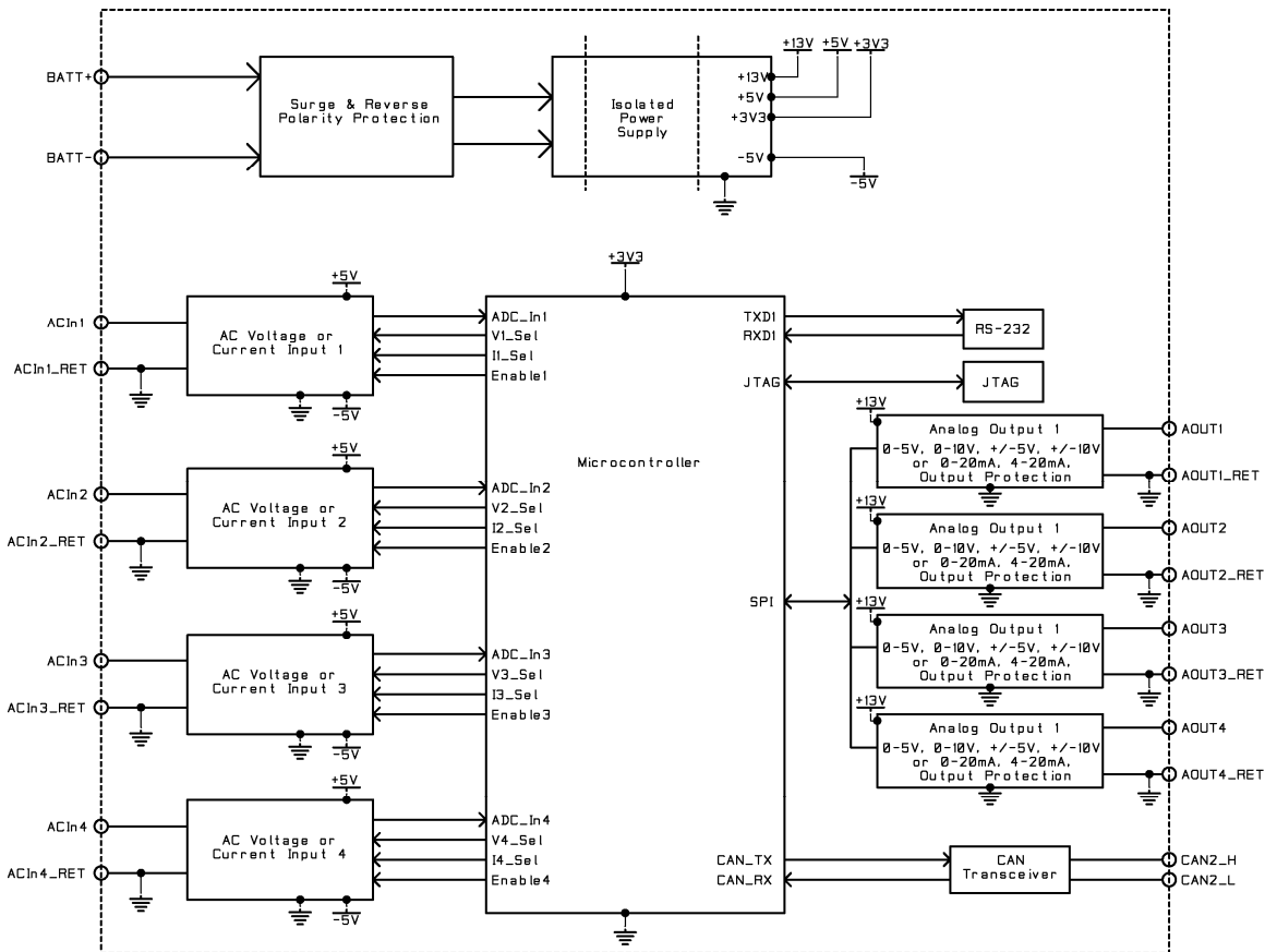
Figure 1.0 – Block Diagram
