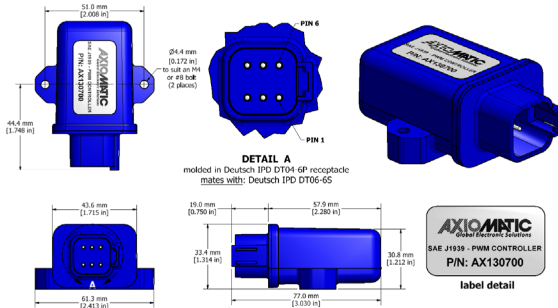
Figure 1.0 – Dimensional Drawing
