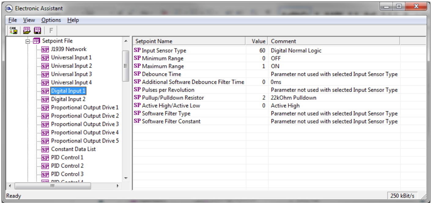
Figure 8 - Screen Capture of Digital Input Setpoints
