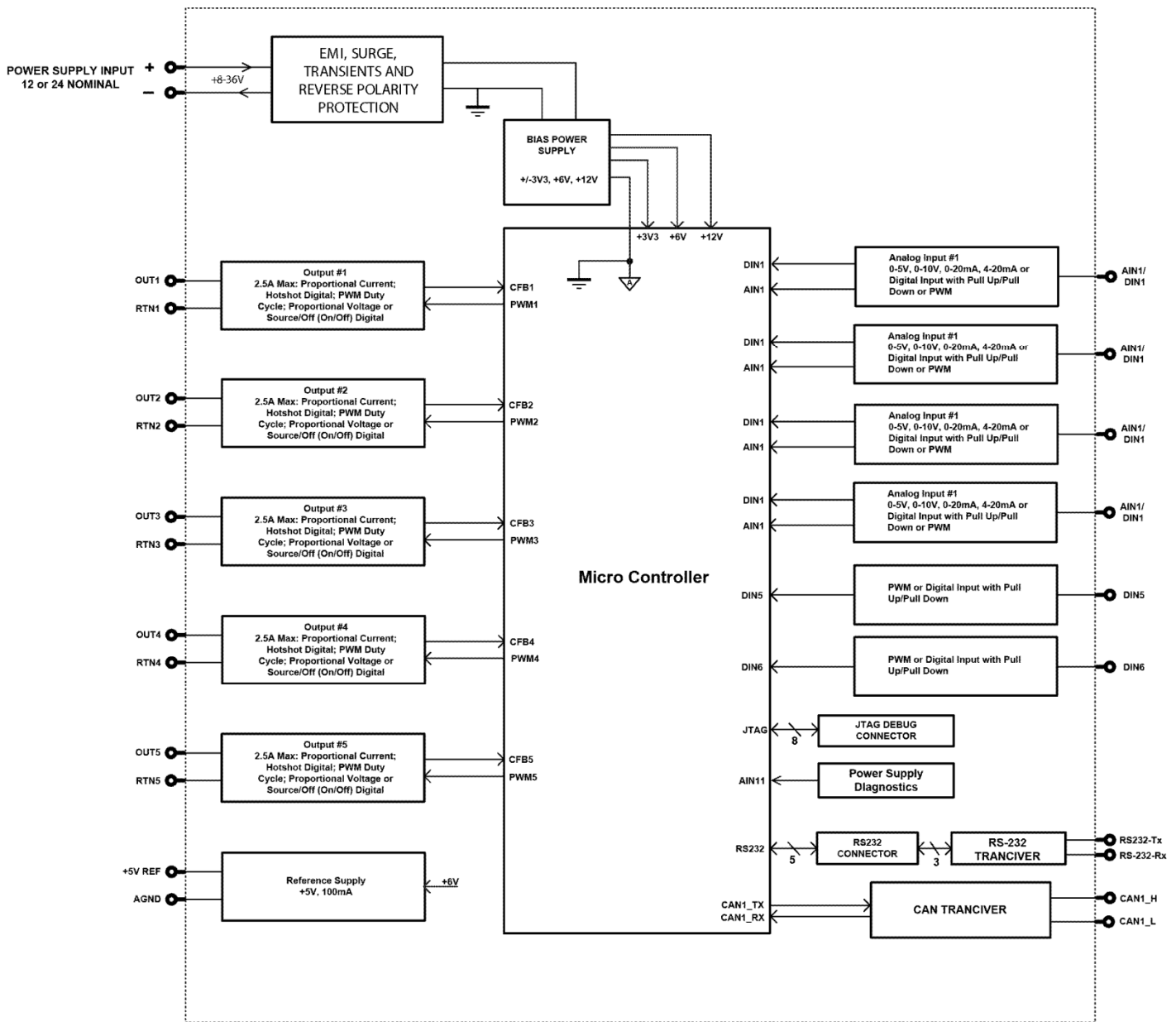
Figure 1 - AX020510 Block Diagram
