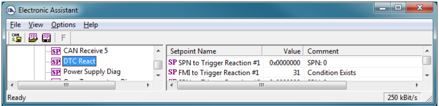
Figure 17 - Screen Capture of DTC React Setpoints
