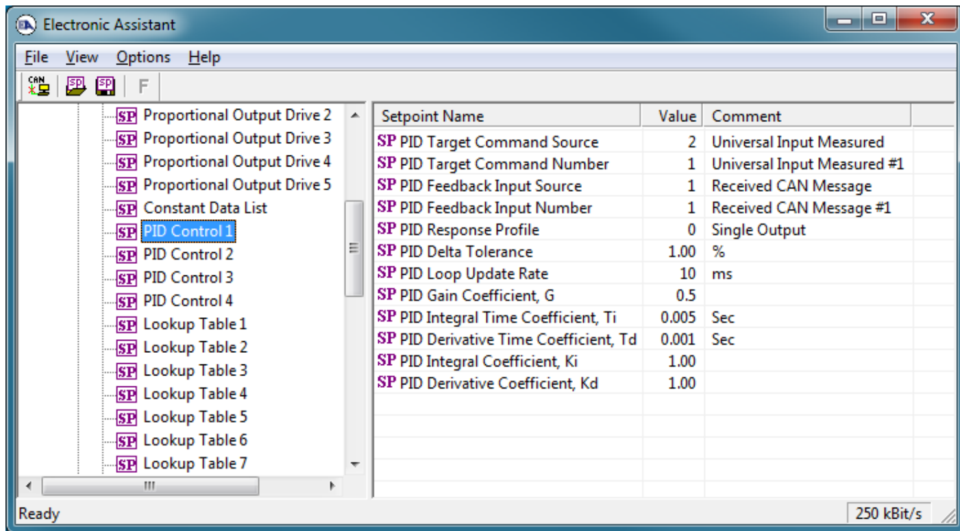
Figure 11 - Screen Capture of PID Control Setpoints
