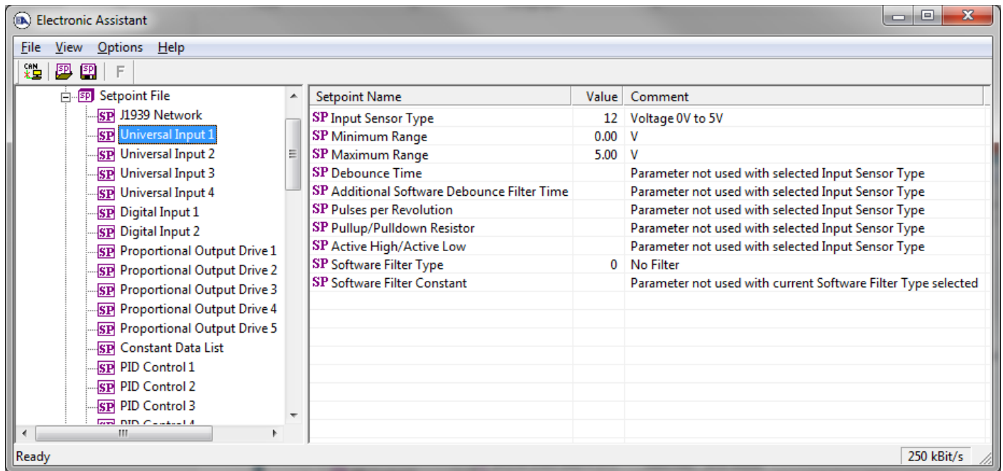
Figure 7 - Screen Capture of Universal Input Setpoints
