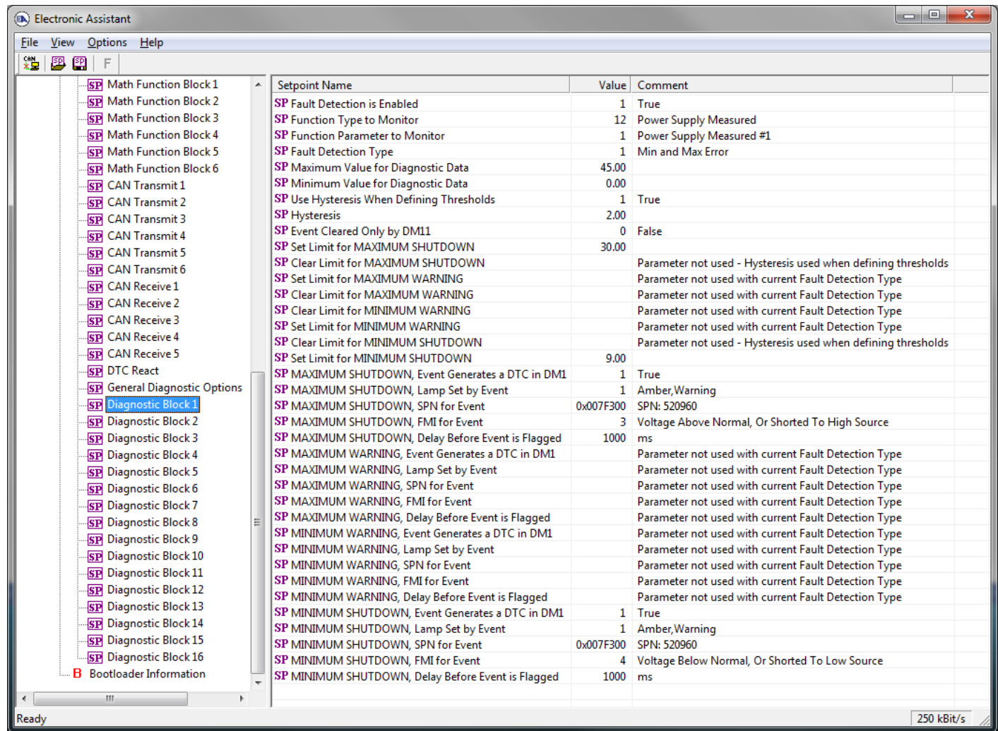
Figure 19 - Screen Capture of Diagnostic Block Setpoints
