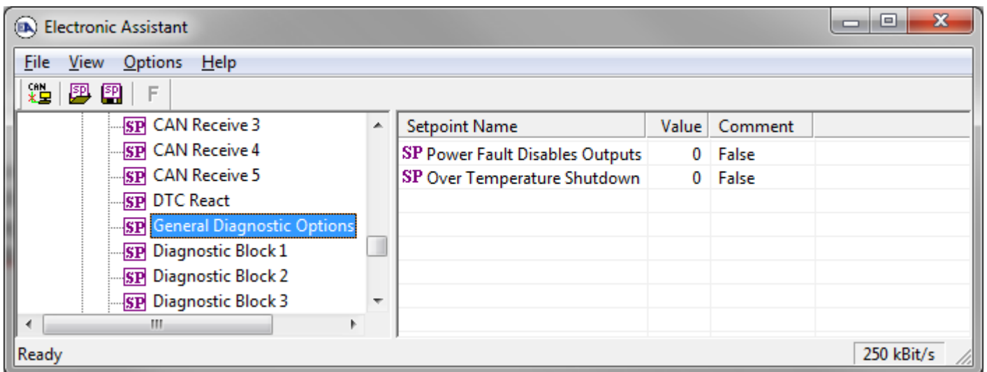
Figure 18 - Screen Capture of General Diagnostics Options Setpoints
