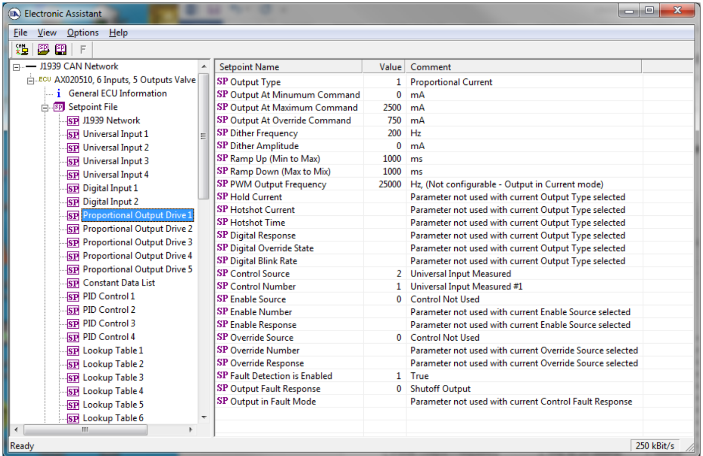
Figure 9 - Screen Capture of Proportional Output Setpoints
