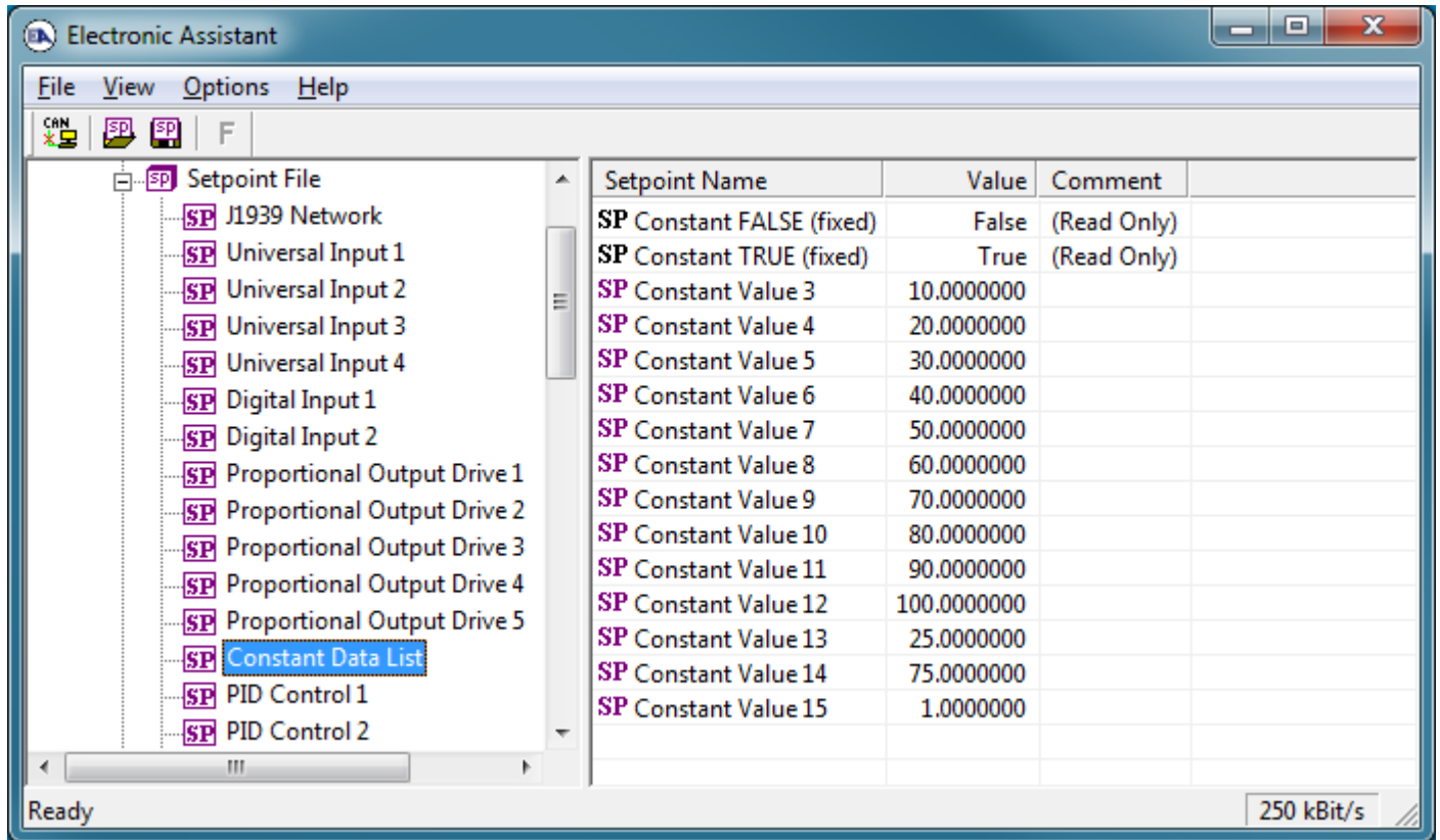
Figure 10 - Screen Capture of Constant Data List Setpoints
