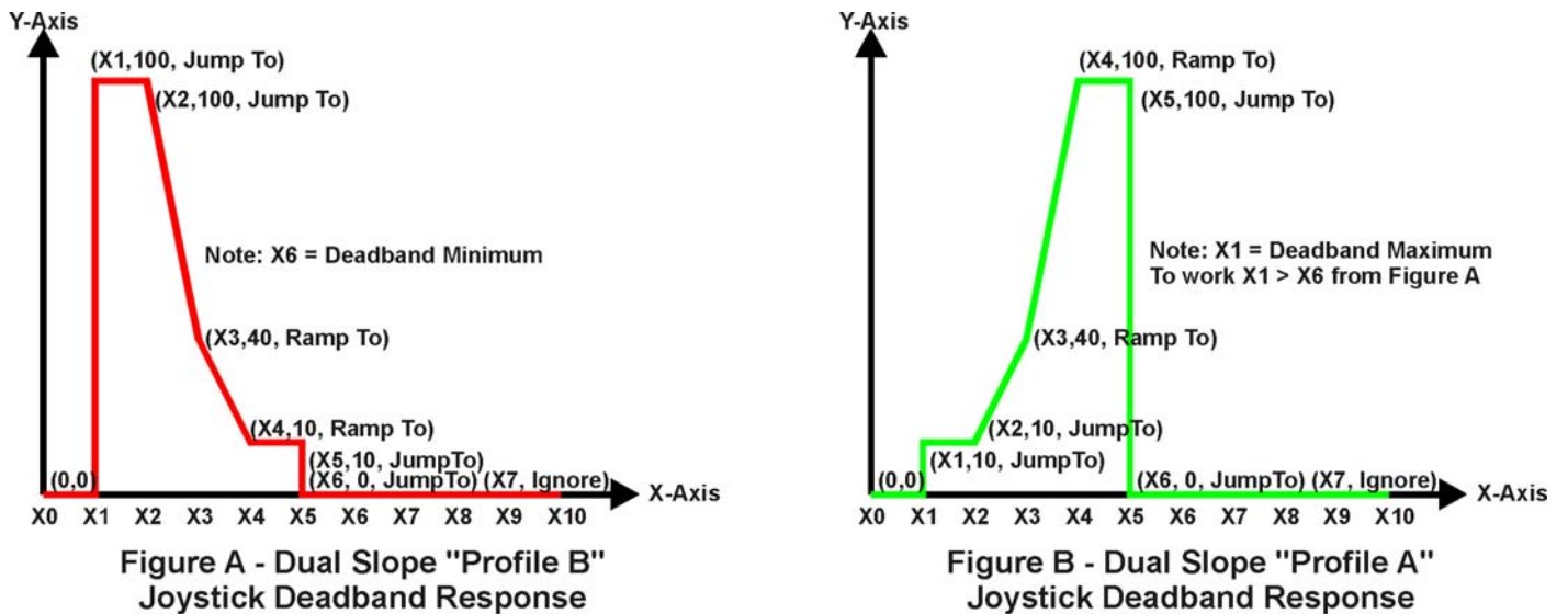
Figure 16 – Lookup Table Examples to Setup for Joystick Deadband Response
