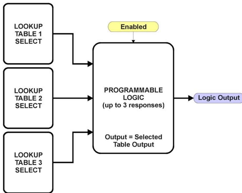
Figure 19 – Programmable Logic Function Block
