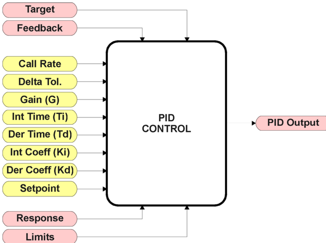
Figure 11 – PID Control Function Block
