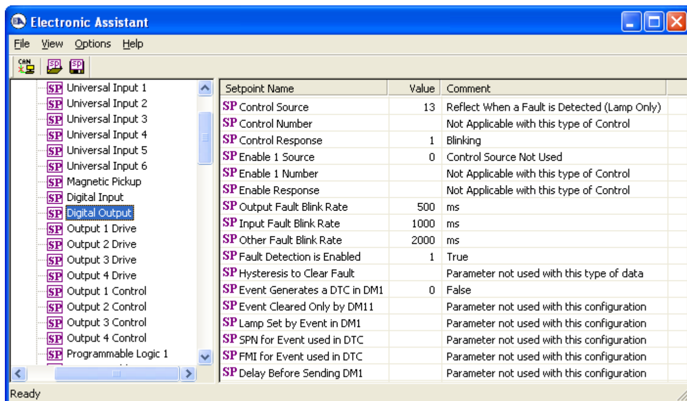
Screen Capture of Default Digital Output Setpoints
