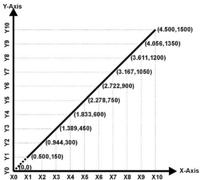
Figure 10: Lookup Table with "Ramp To" Data Response
