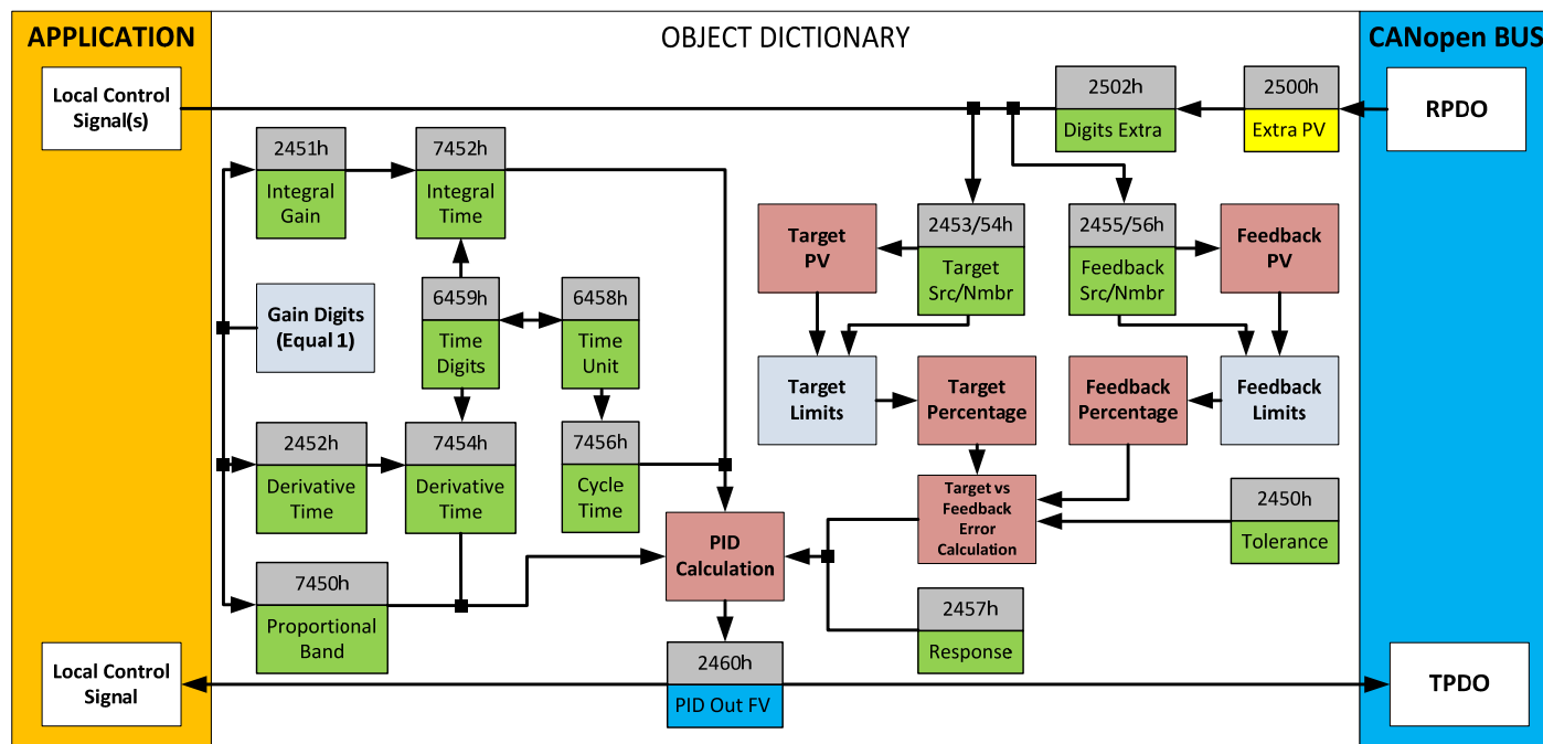
Figure 13: PID Block objects
