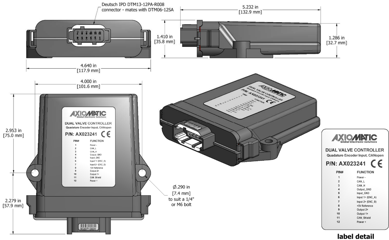
Figure 14: Housing Dimensions
