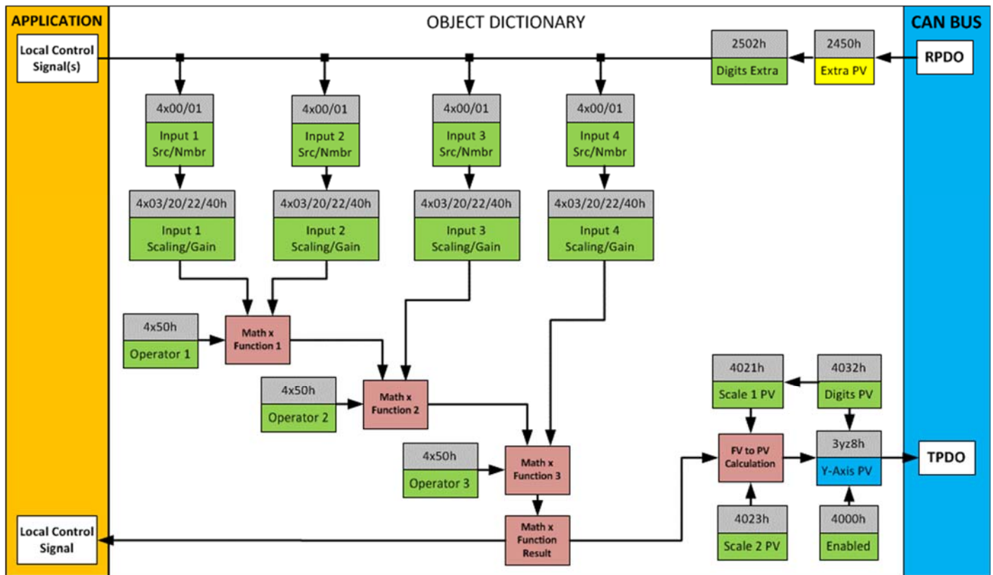
Figure 17 – Math Function Block Objects
