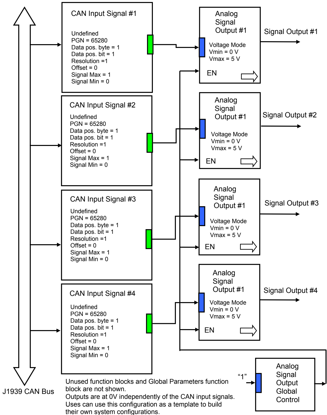
Figure 3. The Block Diagram of the Default Controller Configuration.
