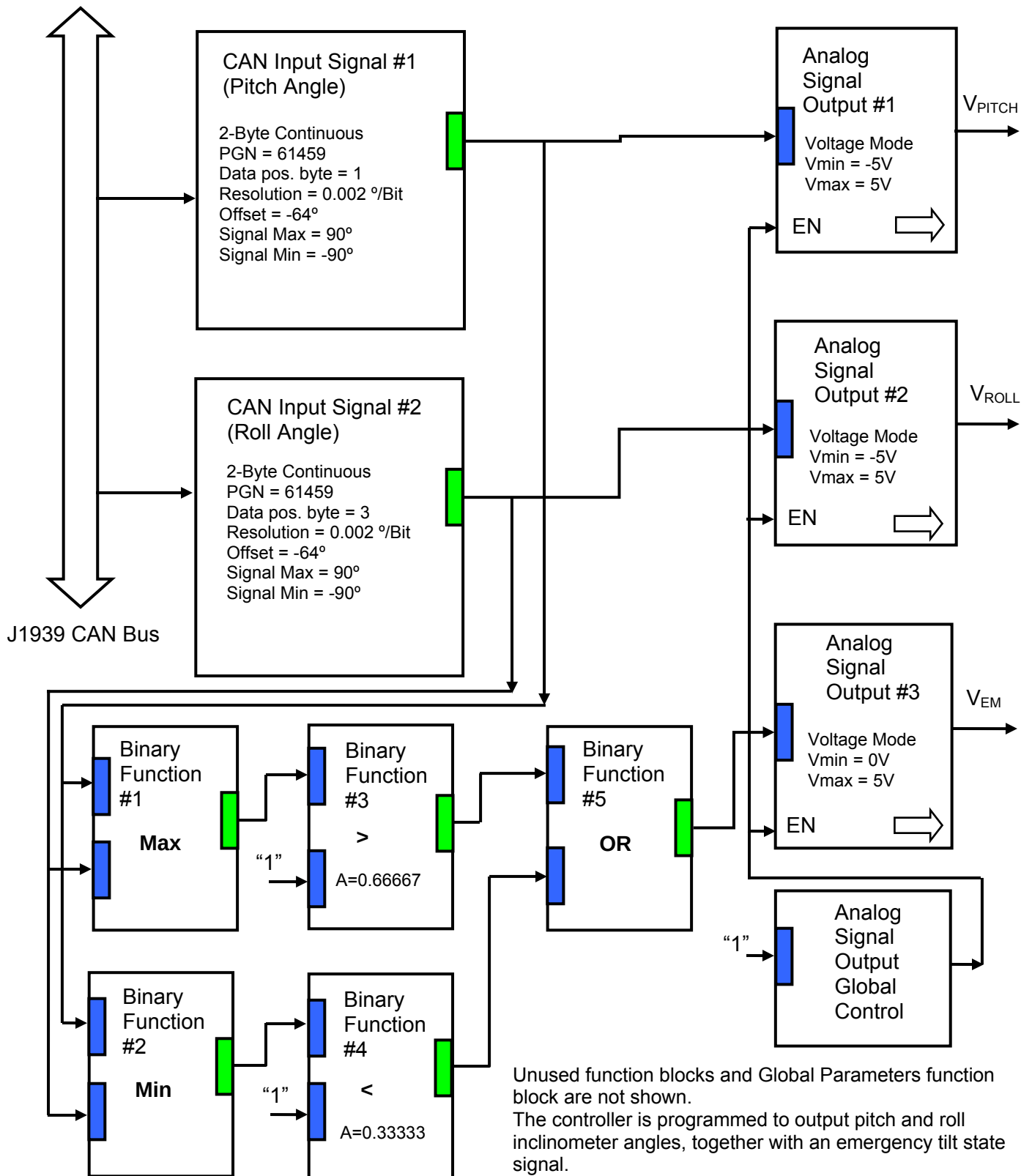
Figure 4. The Block Diagram of the Controller Configuration for the Setpoint Programming Example.
