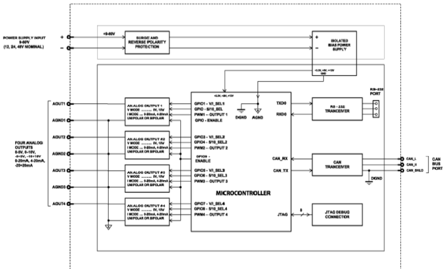
Figure 1. The Controller Hardware Block Diagram.
