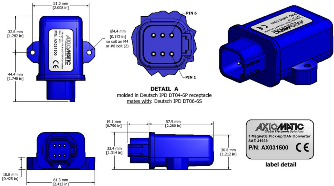
Figure 6 – Housing Dimensions
