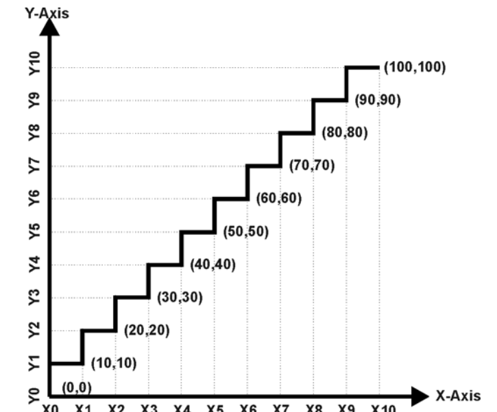
Figure 2 – Lookup Table with “Jump To” Data Response
