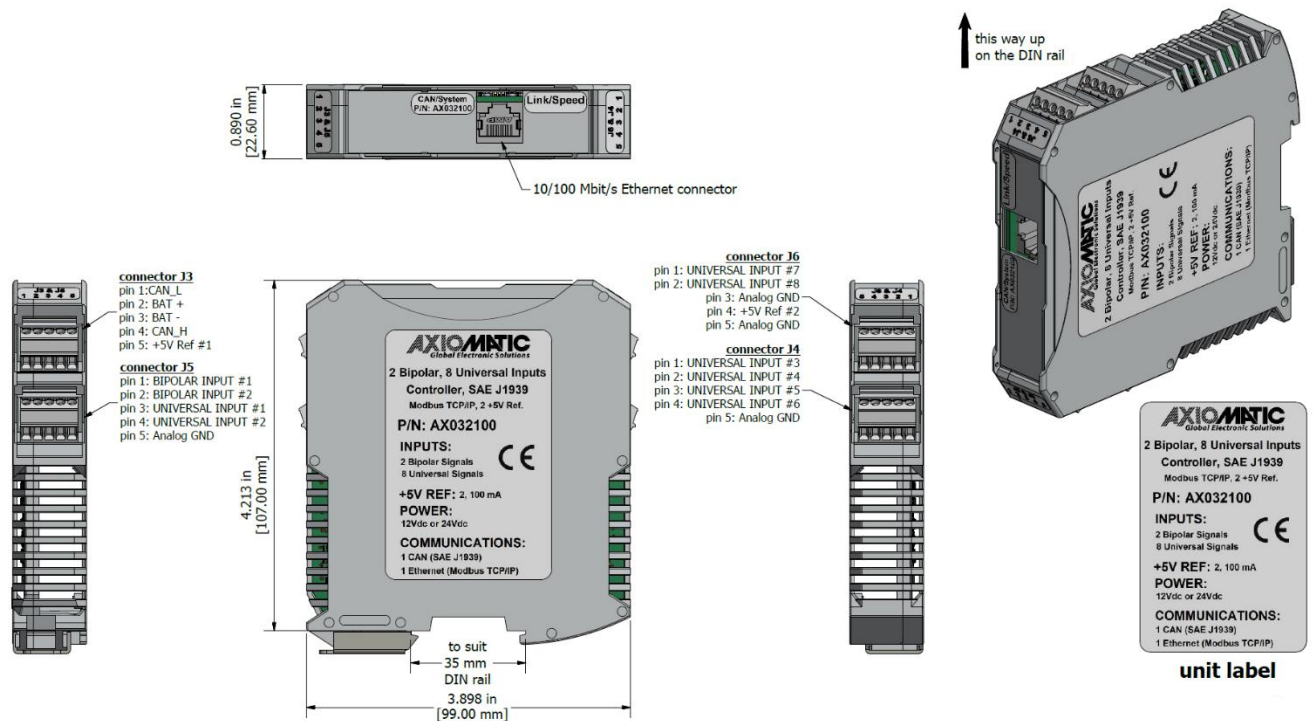
Figure 28. Dimensional Drawing
