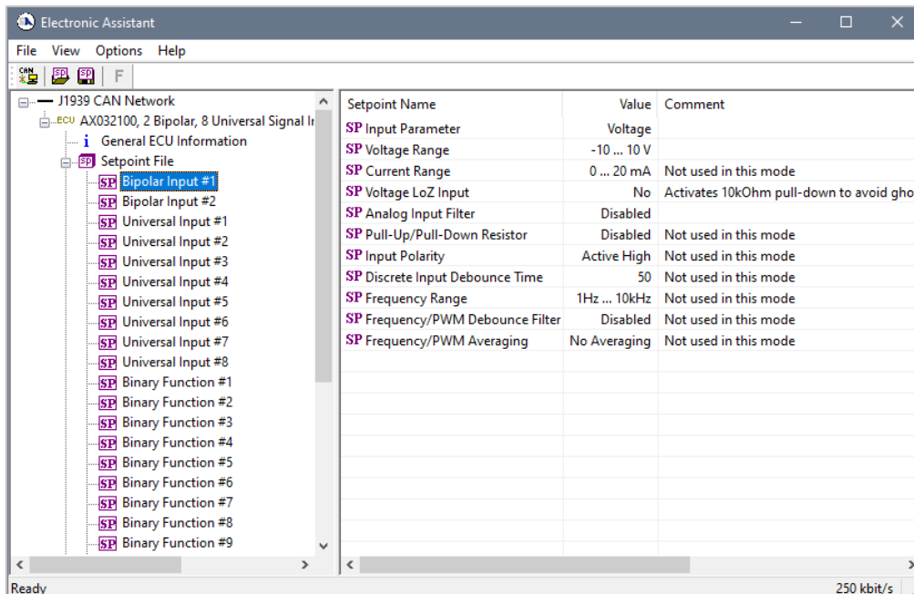
Figure 18. Bipolar Input #1 Example Configuration
