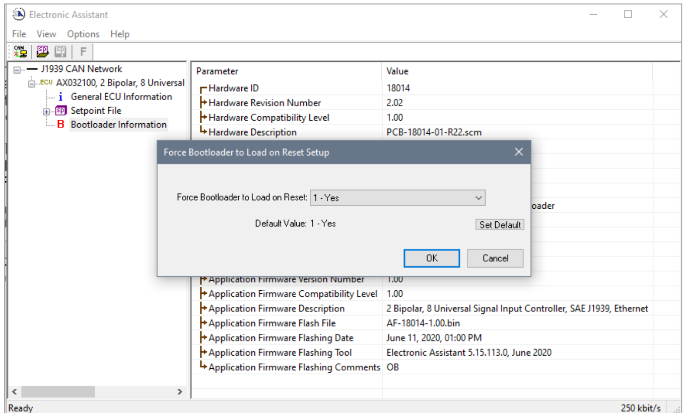
Figure 22. Bootloader Activation. First Step
