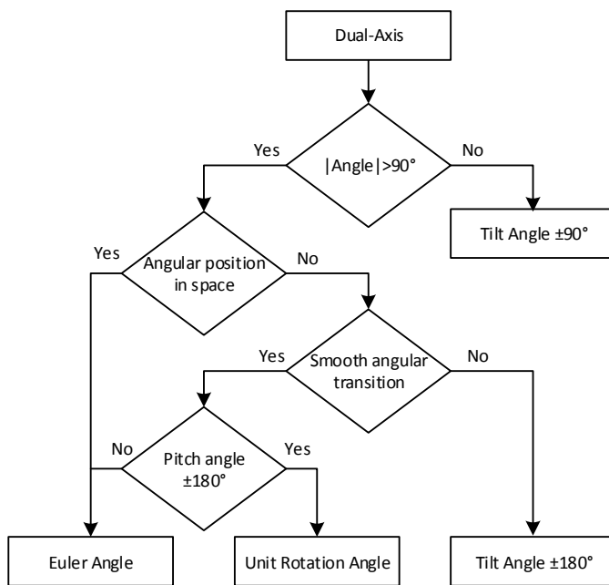
Figure 8. Dual-Axis Measurements
