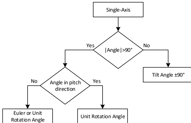
Figure 7. Single-Axis Measurements
