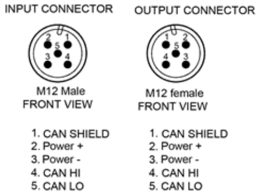
Figure 29. Connector Pinouts
