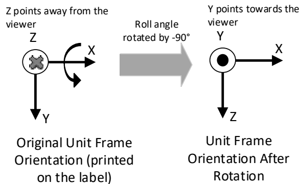
Figure 18. Unit Frame Orientation Example. Coordinate System Rotation
