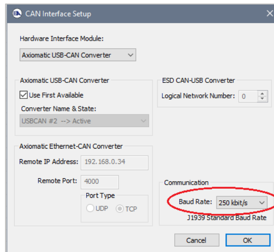
Figure 5-3. CAN Interface Setup Dialog. Baud Rate
