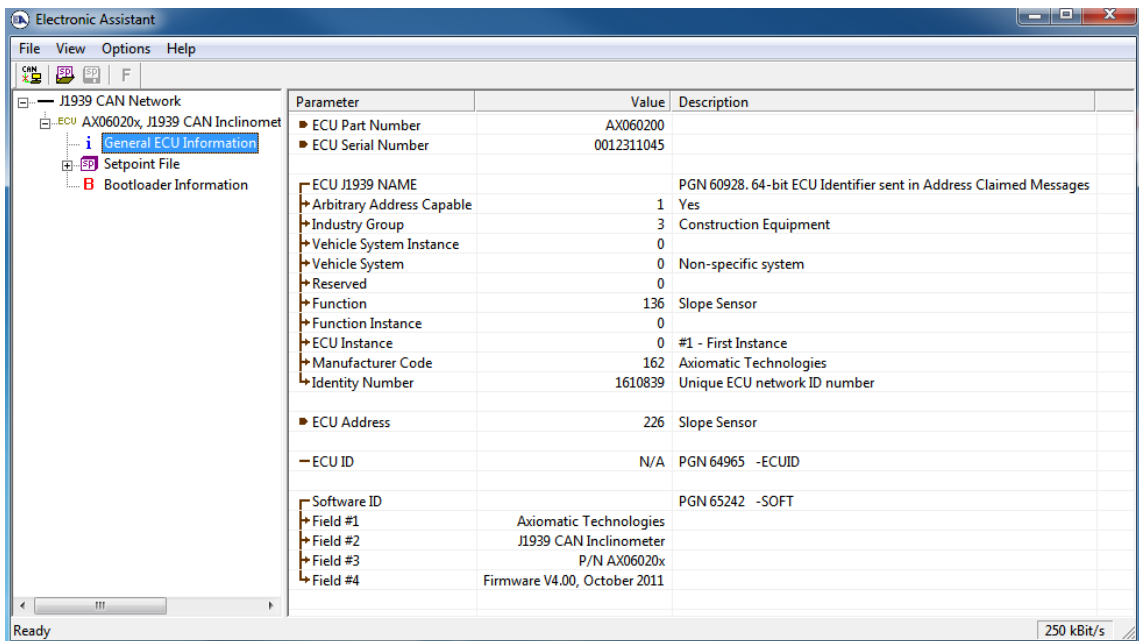
Figure 5-6. General ECU Information (New)
