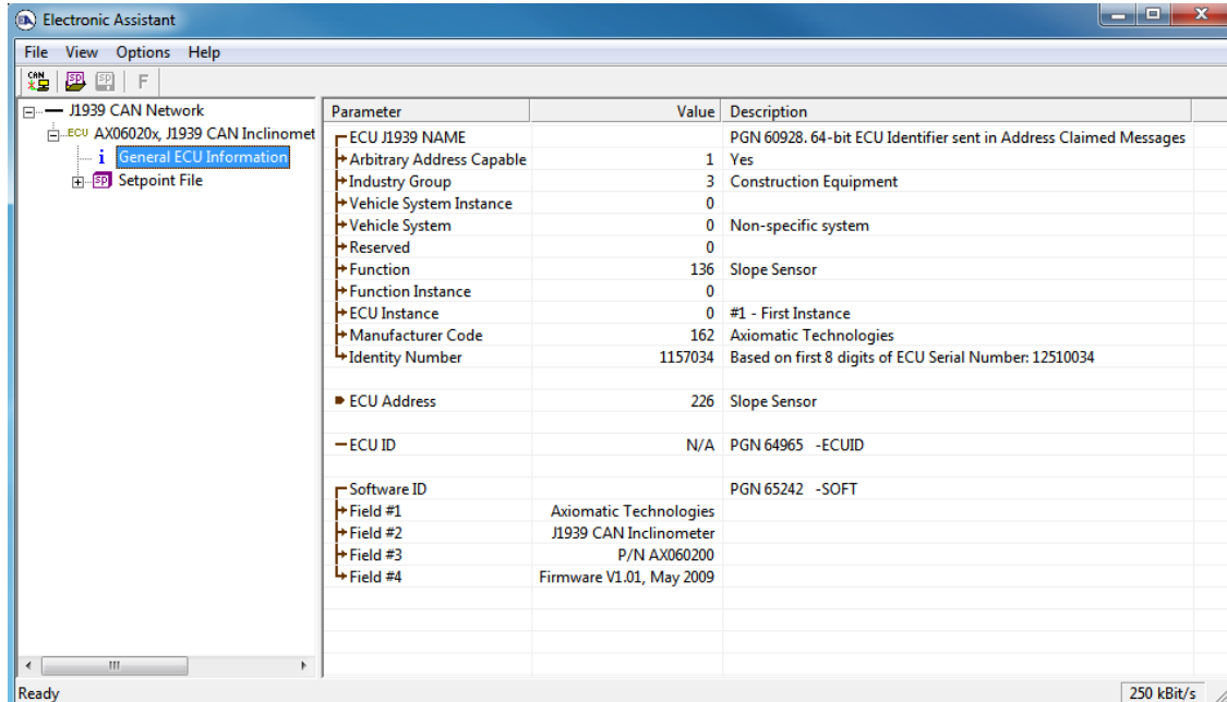
Figure 5-5. General ECU Information
