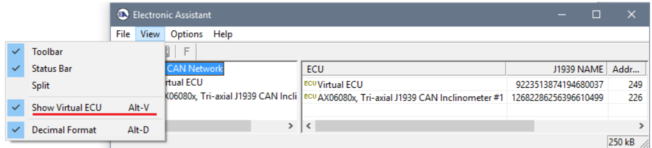
Figure 5-2. Virtual EA ECU
