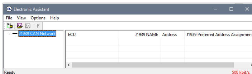
Figure 5-4. CAN bus running at 500 kbit/s baud rate
