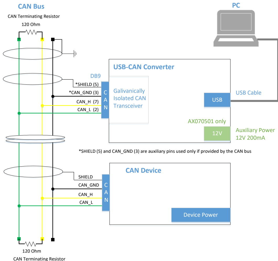
Figure 2-1. Connecting Axiomatic USB-CAN Converter to CAN Bus
