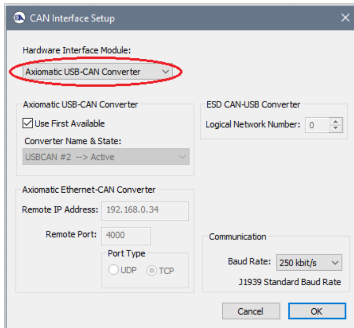
Figure 4-10. CAN Interface Setup Dialog. Setting Hardware Interface Module
