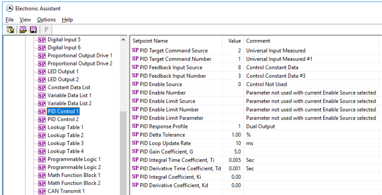
Figure 14 – Screen Capture of PID Control Setpoints
