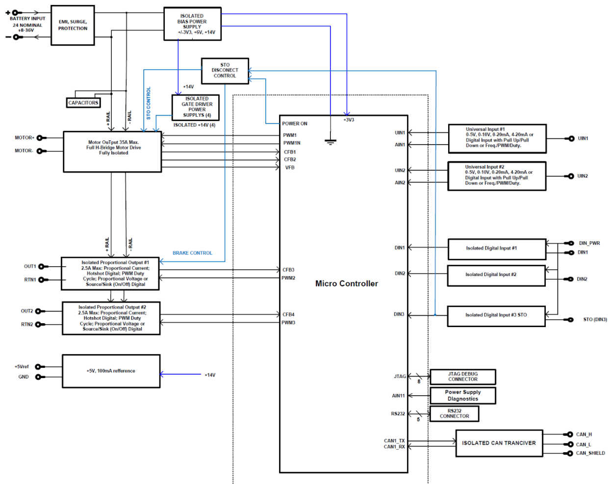
Figure 1 – AX102100 Block Diagram
