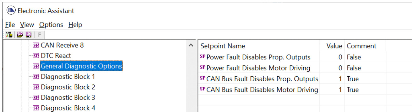
Figure 21 – Screen Capture of General Diagnostics Options Setpoints
