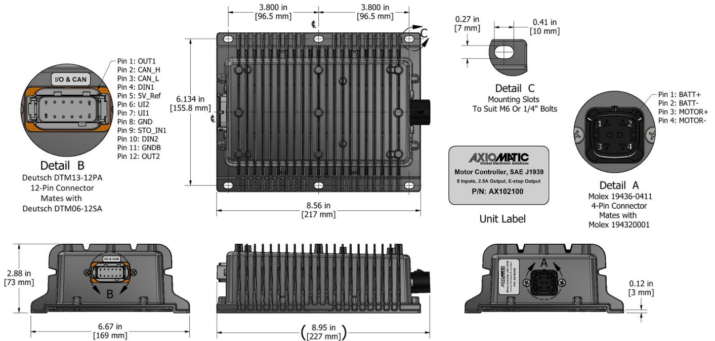
Figure 5 – AX102100 Dimensional Drawing
