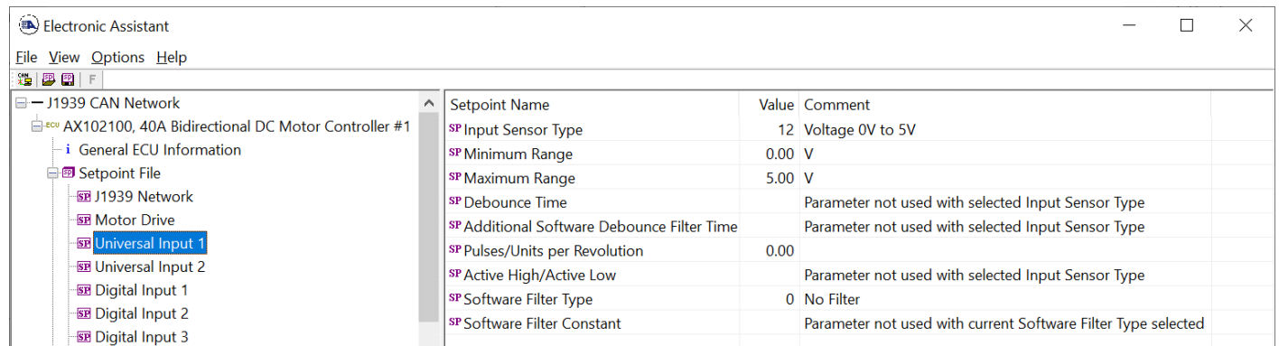
Figure 8 – Screen Capture of Universal Input Setpoints
