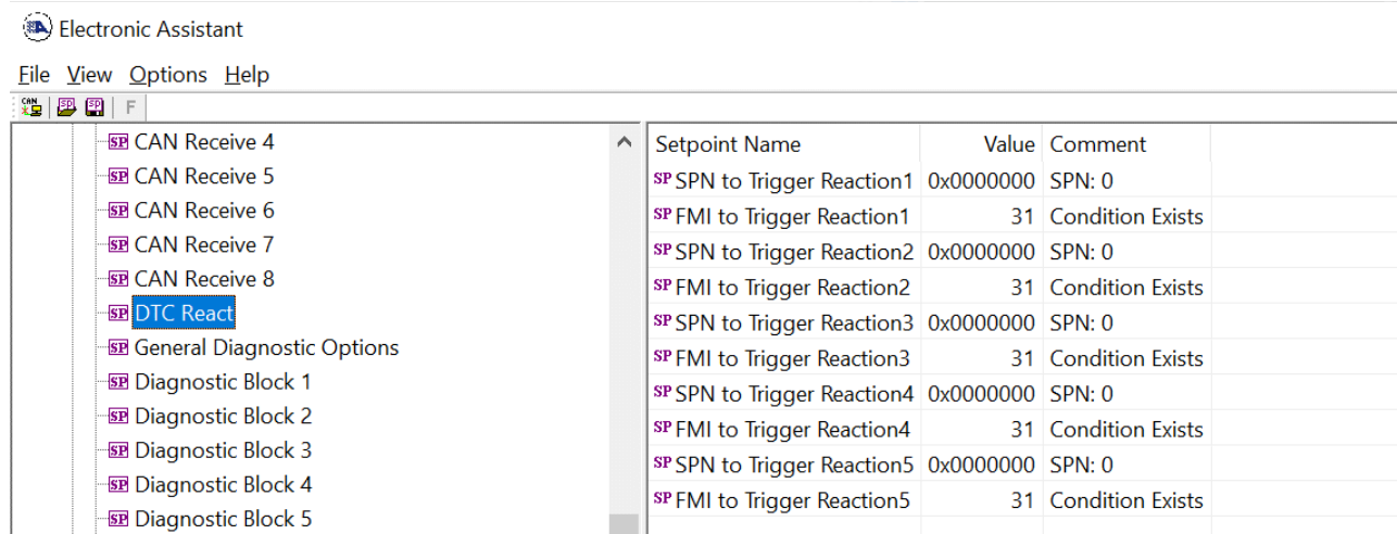
Figure 20 – Screen Capture of DTC React Setpoints
