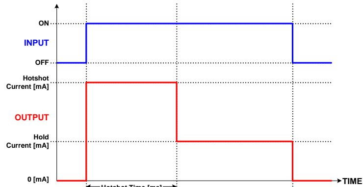
Figure 1 – Proportional Output Hotshot Digital Profile
