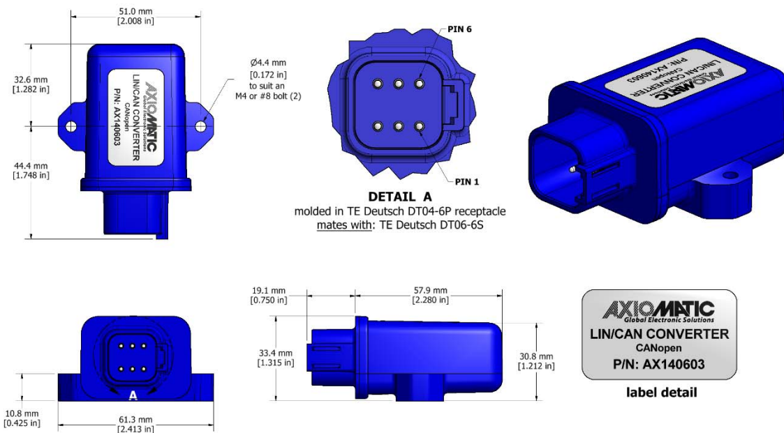
Figure 17. Unit Dimensions
