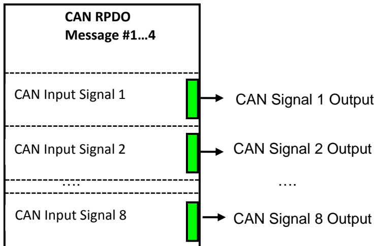
Figure 14. CAN Input Signal Function Block
