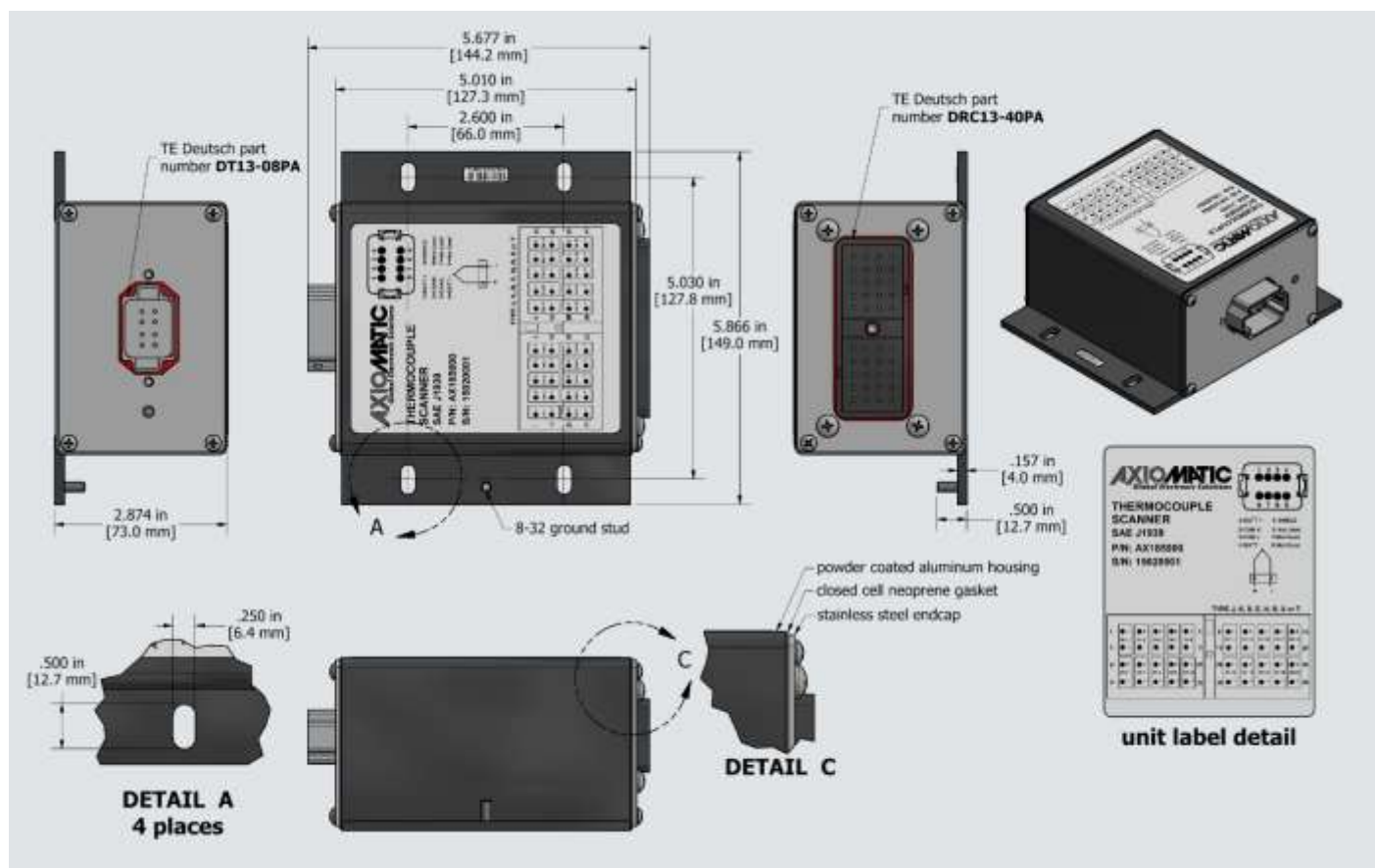
Figure 4 – AX185000 Dimensional Drawing
