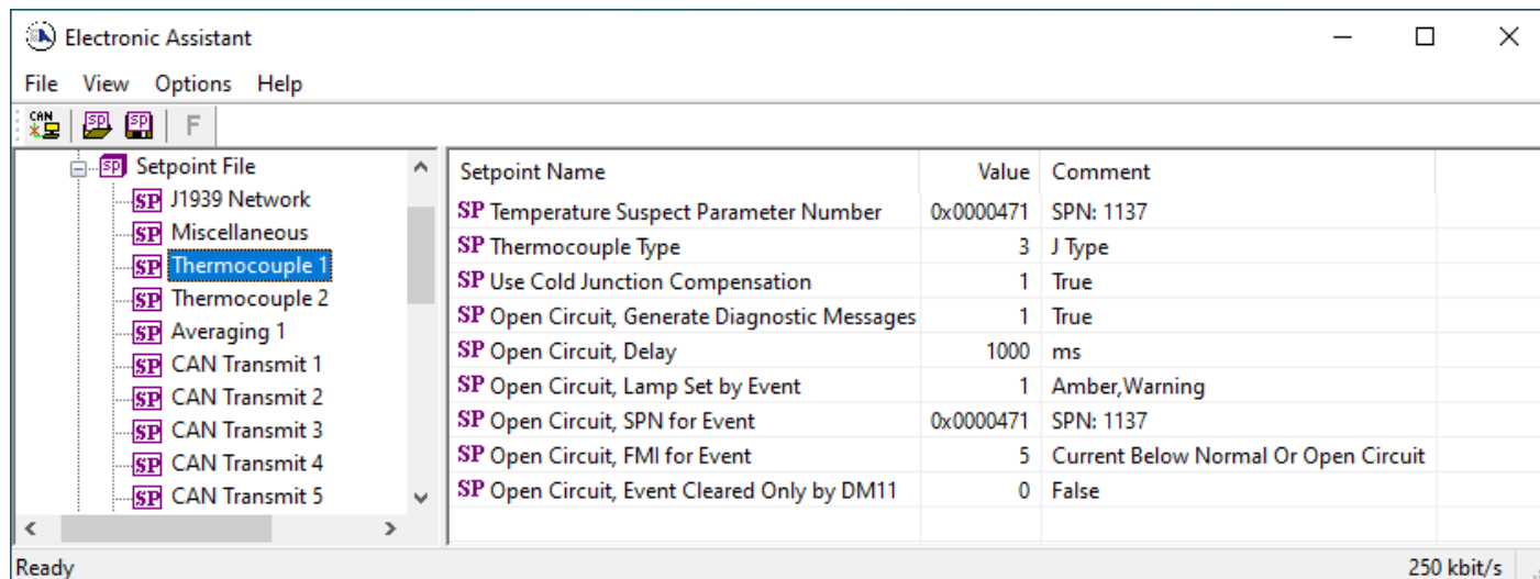
Figure 8 – Screen Capture of TC Input Setpoints
